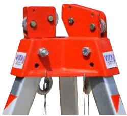
(01) Tripod 7FT or 10FT Double Pulley Head SF-TP-800(DP)
